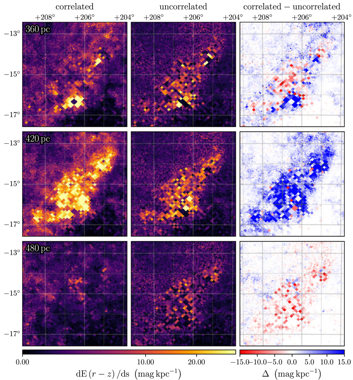
Figure 8. from A 3D Dust Map Based on Gaia, Pan-STARRS 1, and 2MASS null 2019 APJ 887 93 doi:10.3847/1538-4357/ab5362 https://dx.doi.org/10.3847/1538-4357/ab5362 © 2019. The American Astronomical Society. All rights reserved.
