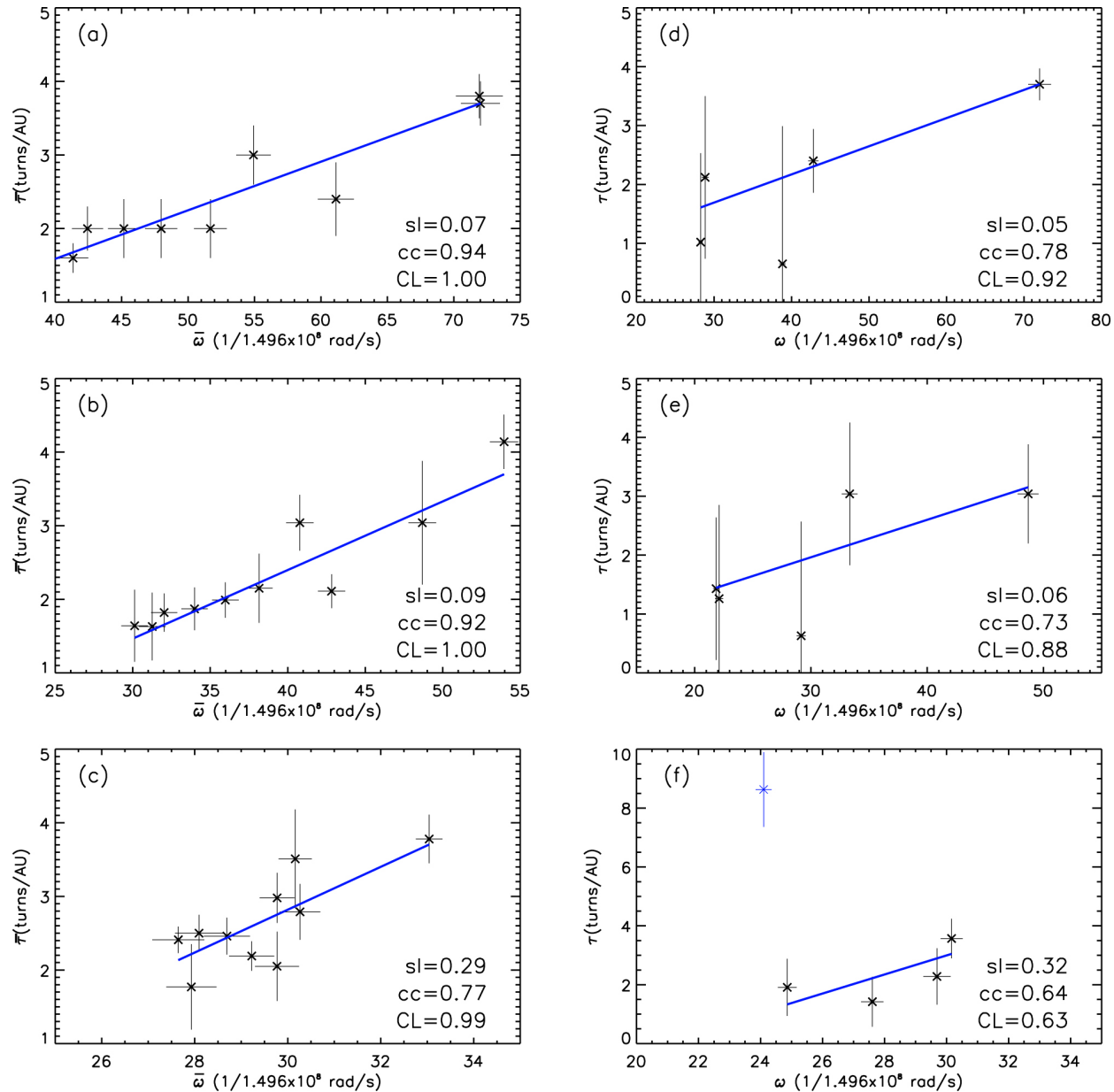
Figure 2. from The Relationship of Magnetic Twist and Plasma Motion in a Magnetic Cloud null 2019 APJ 885 122 doi:10.3847/1538-4357/ab48e5 https://dx.doi.org/10.3847/1538-4357/ab48e5 © 2019. The American Astronomical Society. All rights reserved.
