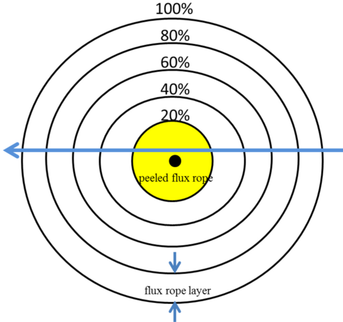
Figure 1. from The Relationship of Magnetic Twist and Plasma Motion in a Magnetic Cloud null 2019 APJ 885 122 doi:10.3847/1538-4357/ab48e5 https://dx.doi.org/10.3847/1538-4357/ab48e5 © 2019. The American Astronomical Society. All rights reserved.
