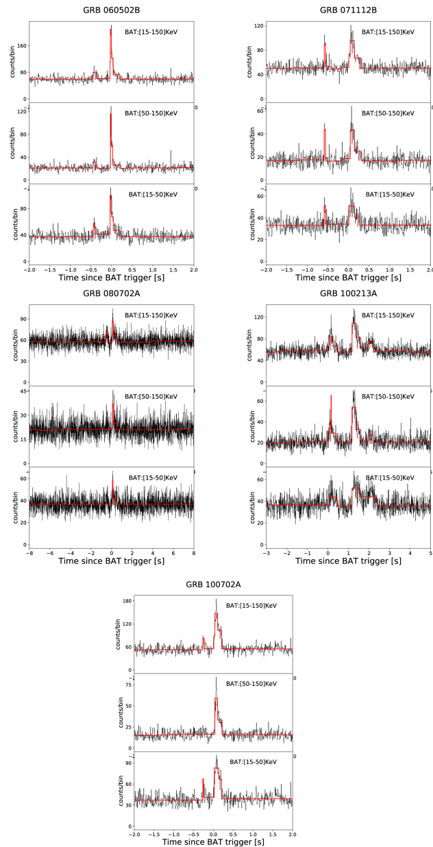
Figure 1. from Precursors in Short Gamma-Ray Bursts as a Possible Probe of Progenitors null 2019 APJ 884 25 doi:10.3847/1538-4357/ab3e48 https://dx.doi.org/10.3847/1538-4357/ab3e48 © 2019. The American Astronomical Society. All rights reserved.
