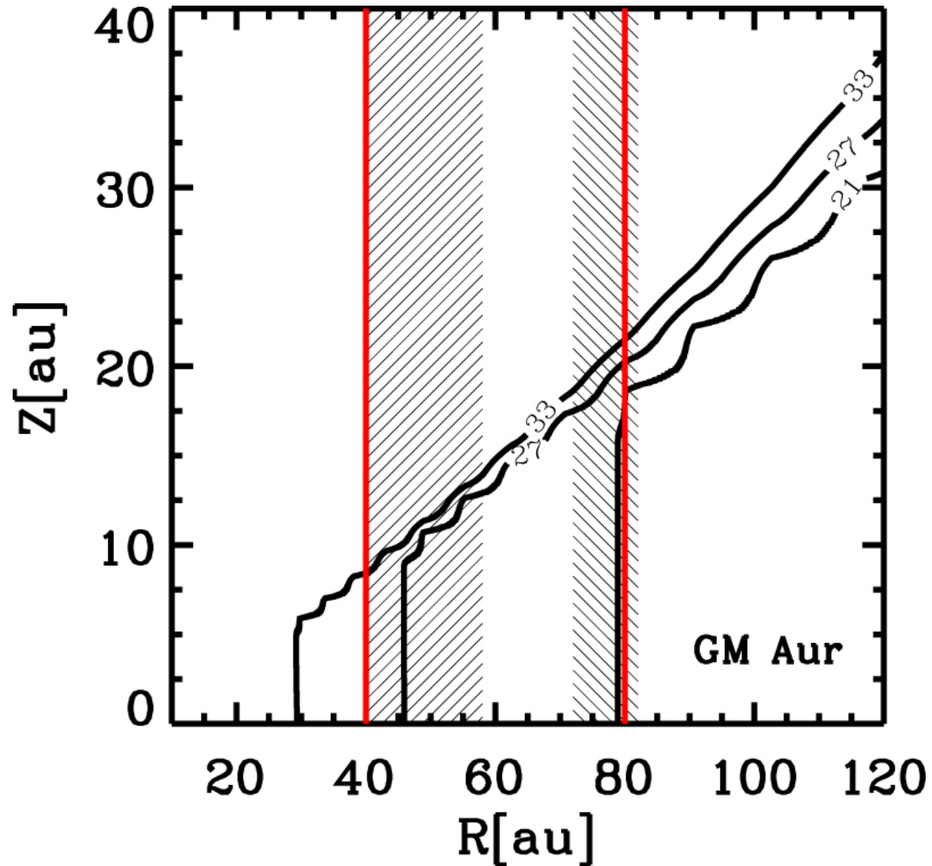
Figure 9. from Probing CO and N 2 Snow Surfaces in Protoplanetary Disks with N 2 H + Emission null 2019 APJ 882 160 doi:10.3847/1538-4357/ab35d3 https://dx.doi.org/10.3847/1538-4357/ab35d3 © 2019. The American Astronomical Society. All rights reserved.
