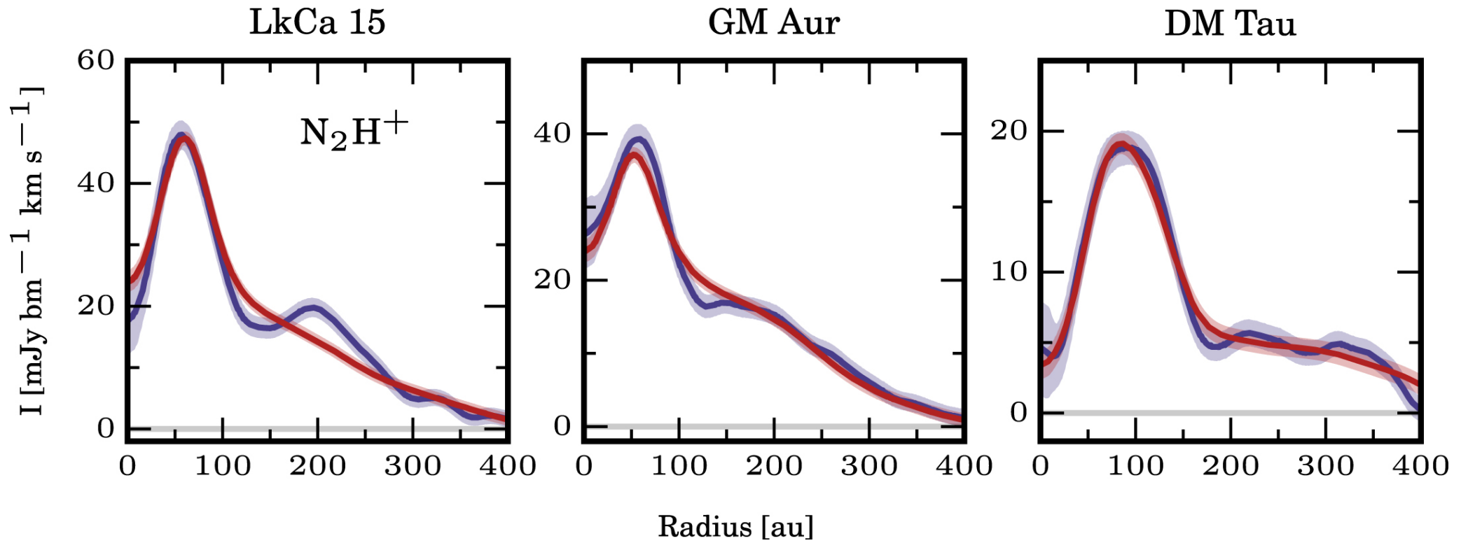
Figure 8. from Probing CO and N 2 Snow Surfaces in Protoplanetary Disks with N 2 H + Emission null 2019 APJ 882 160 doi:10.3847/1538-4357/ab35d3 https://dx.doi.org/10.3847/1538-4357/ab35d3 © 2019. The American Astronomical Society. All rights reserved.
