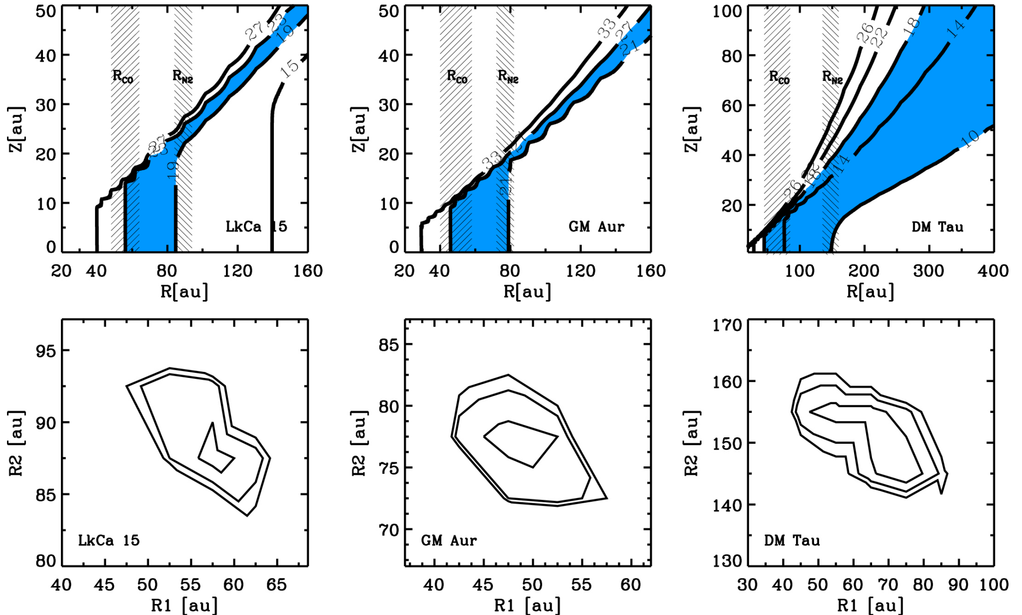
Figure 7. from Probing CO and N 2 Snow Surfaces in Protoplanetary Disks with N 2 H + Emission null 2019 APJ 882 160 doi:10.3847/1538-4357/ab35d3 https://dx.doi.org/10.3847/1538-4357/ab35d3 © 2019. The American Astronomical Society. All rights reserved.
