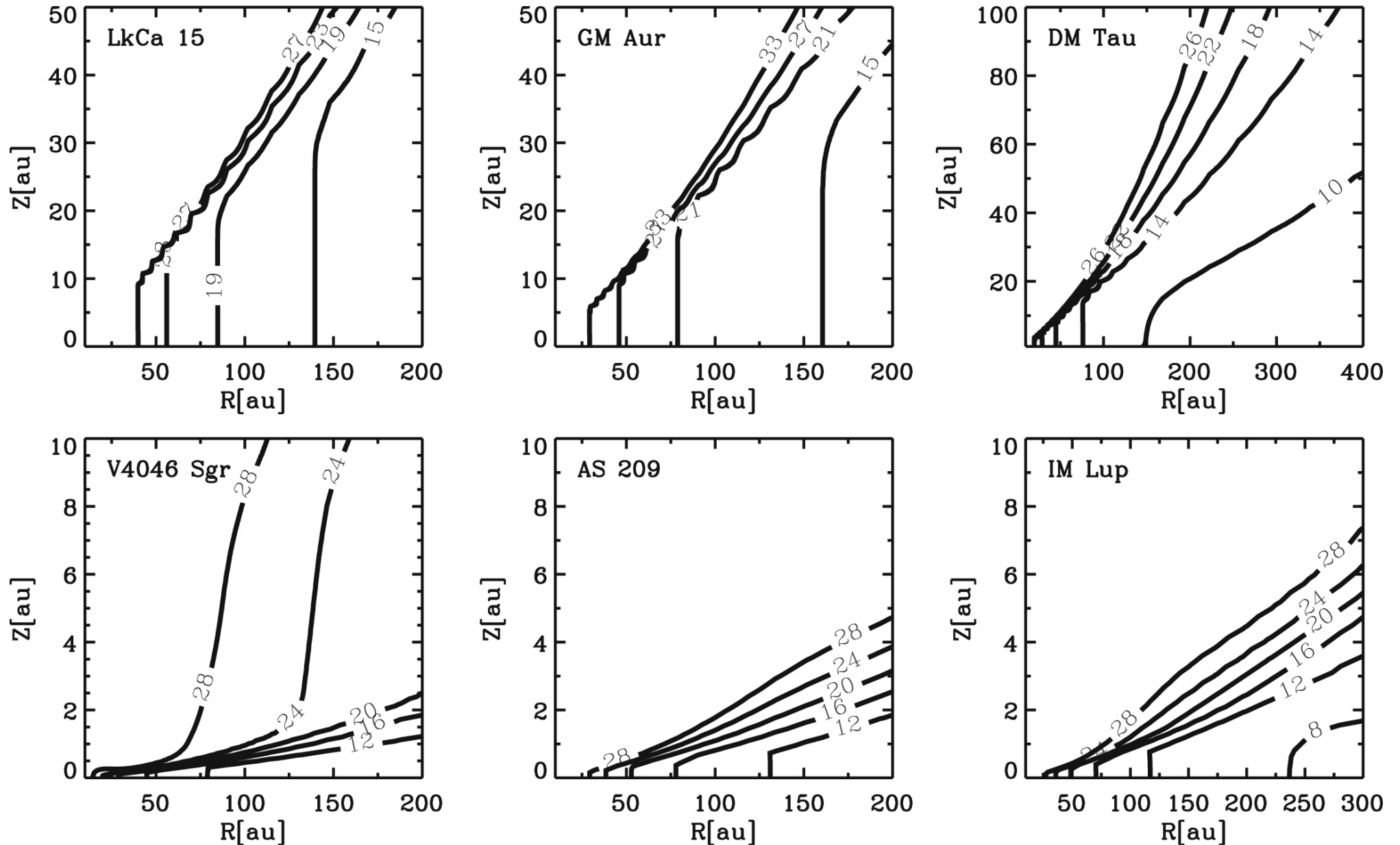
Figure 5. from Probing CO and N 2 Snow Surfaces in Protoplanetary Disks with N 2 H + Emission null 2019 APJ 882 160 doi:10.3847/1538-4357/ab35d3 https://dx.doi.org/10.3847/1538-4357/ab35d3
