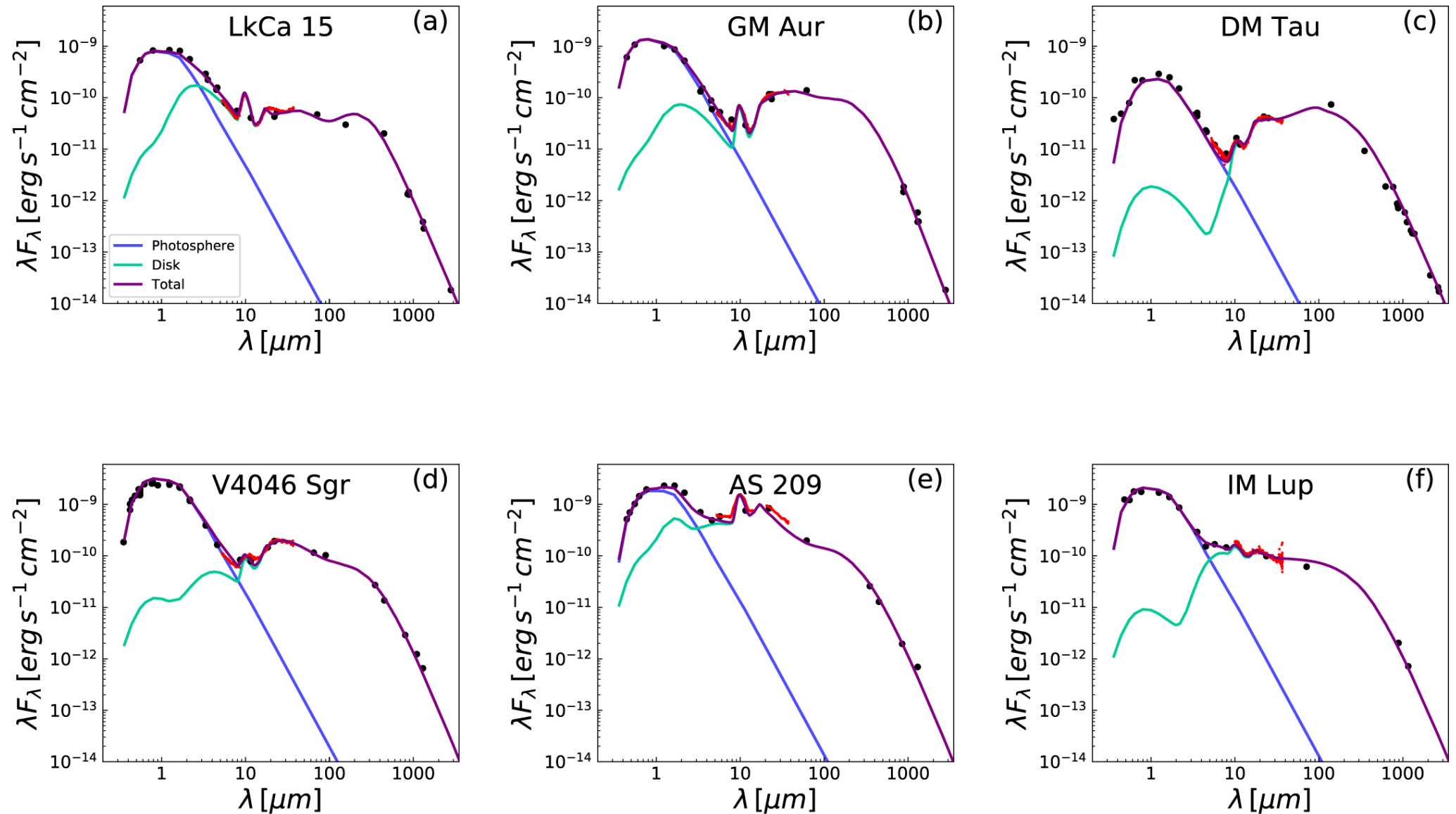
Figure 4. from Probing CO and N 2 Snow Surfaces in Protoplanetary Disks with N 2 H + Emission null 2019 APJ 882 160 doi:10.3847/1538-4357/ab35d3 https://dx.doi.org/10.3847/1538-4357/ab35d3 © 2019. The American Astronomical Society. All rights reserved.
