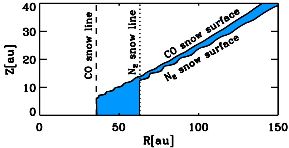
Figure 3. from Probing CO and N 2 Snow Surfaces in Protoplanetary Disks with N 2 H + Emission null 2019 APJ 882 160 doi:10.3847/1538-4357/ab35d3 https://dx.doi.org/10.3847/1538-4357/ab35d3 © 2019. The American Astronomical Society. All rights reserved.
