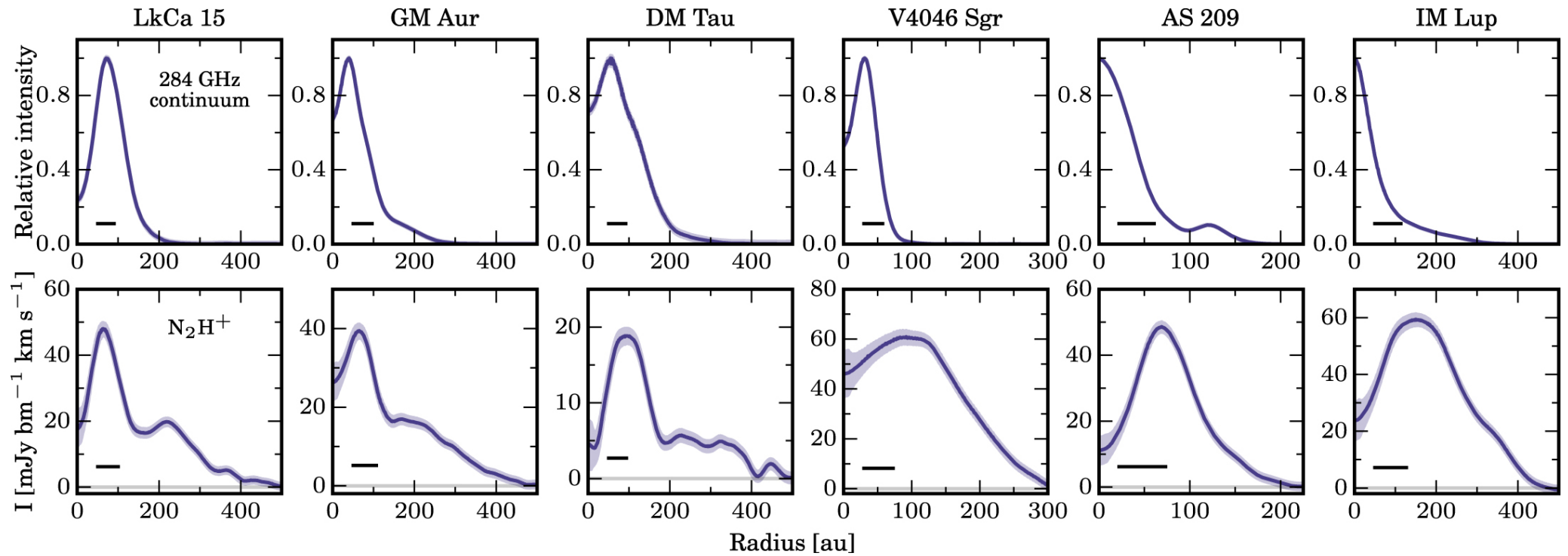
Figure 2. from Probing CO and N 2 Snow Surfaces in Protoplanetary Disks with N 2 H + Emission null 2019 APJ 882 160 doi:10.3847/1538-4357/ab35d3 https://dx.doi.org/10.3847/1538-4357/ab35d3 © 2019. The American Astronomical Society. All rights reserved.
