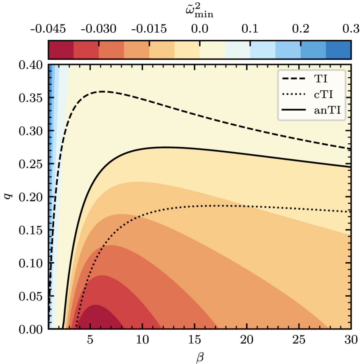
Figure 3. from The Tayler Instability in the Anelastic Approximation null 2019 APJ 881 66 doi:10.3847/1538-4357/ab2a11 https://dx.doi.org/10.3847/1538-4357/ab2a11 © 2019. The American Astronomical Society. All rights reserved.
