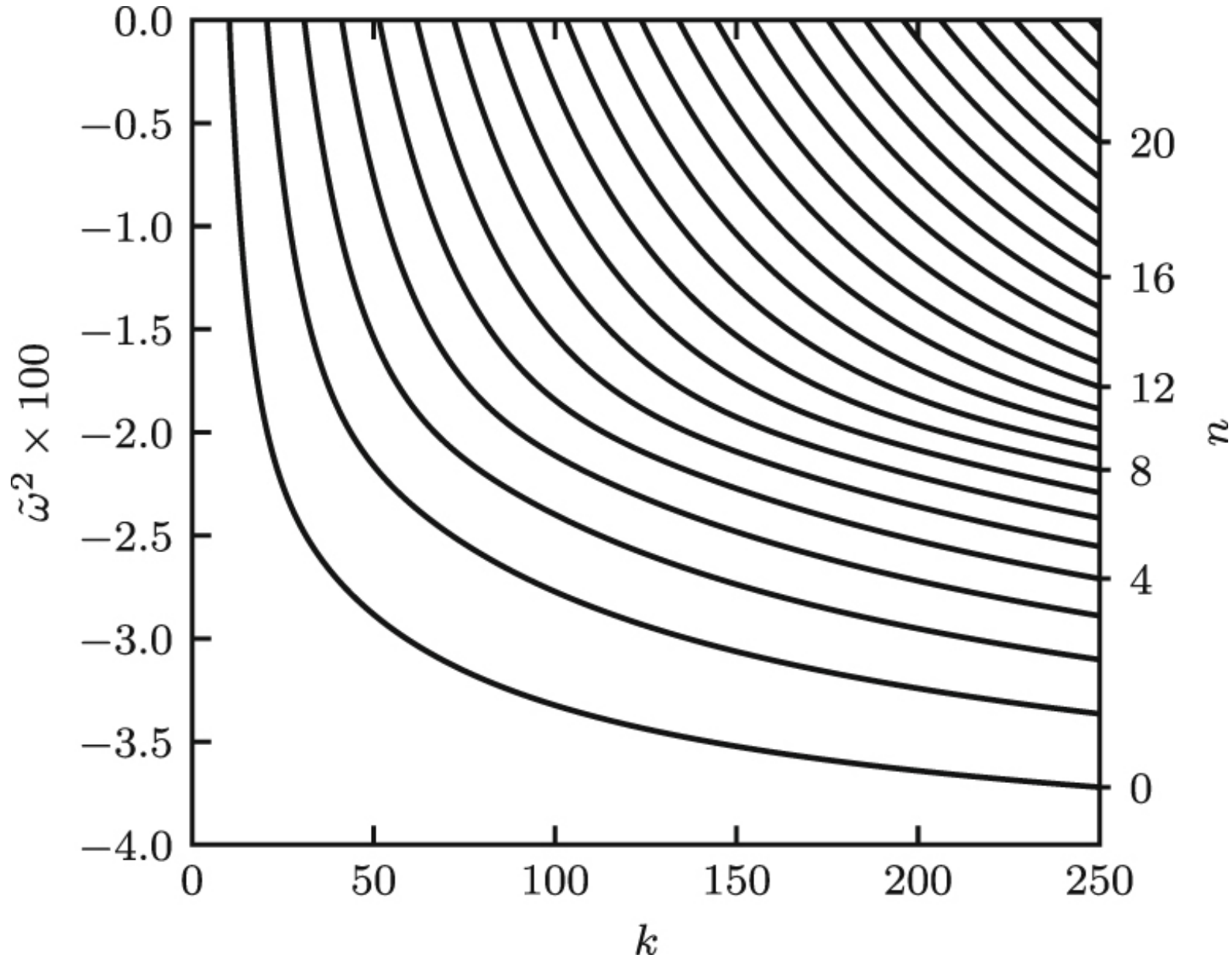
Figure 2. from The Tayler Instability in the Anelastic Approximation null 2019 APJ 881 66 doi:10.3847/1538-4357/ab2a11 https://dx.doi.org/10.3847/1538-4357/ab2a11 © 2019. The American Astronomical Society. All rights reserved.
