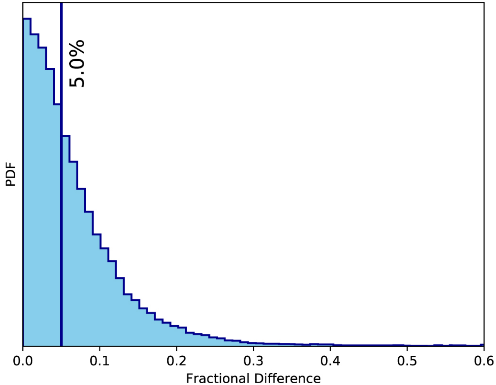
Figure 9. from A Large Catalog of Accurate Distances to Local Molecular Clouds: The Gaia DR2 Edition null 2019 APJ 879 125 doi:10.3847/1538-4357/ab2388 https://dx.doi.org/10.3847/1538-4357/ab2388 © 2019. The American Astronomical Society. All rights reserved.
