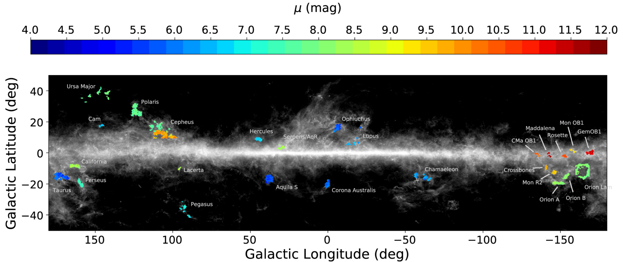
Figure 8. from A Large Catalog of Accurate Distances to Local Molecular Clouds: The Gaia DR2 Edition null 2019 APJ 879 125 doi:10.3847/1538-4357/ab2388 https://dx.doi.org/10.3847/1538-4357/ab2388 © 2019. The American Astronomical Society. All rights reserved.
