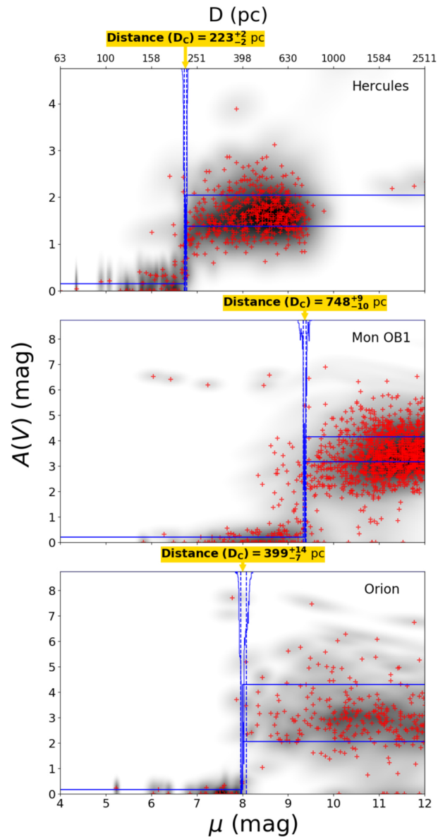
Figure 3. from A Large Catalog of Accurate Distances to Local Molecular Clouds: The Gaia DR2 Edition null 2019 APJ 879 125 doi:10.3847/1538-4357/ab2388 https://dx.doi.org/10.3847/1538-4357/ab2388 © 2019. The American Astronomical Society. All rights reserved.
