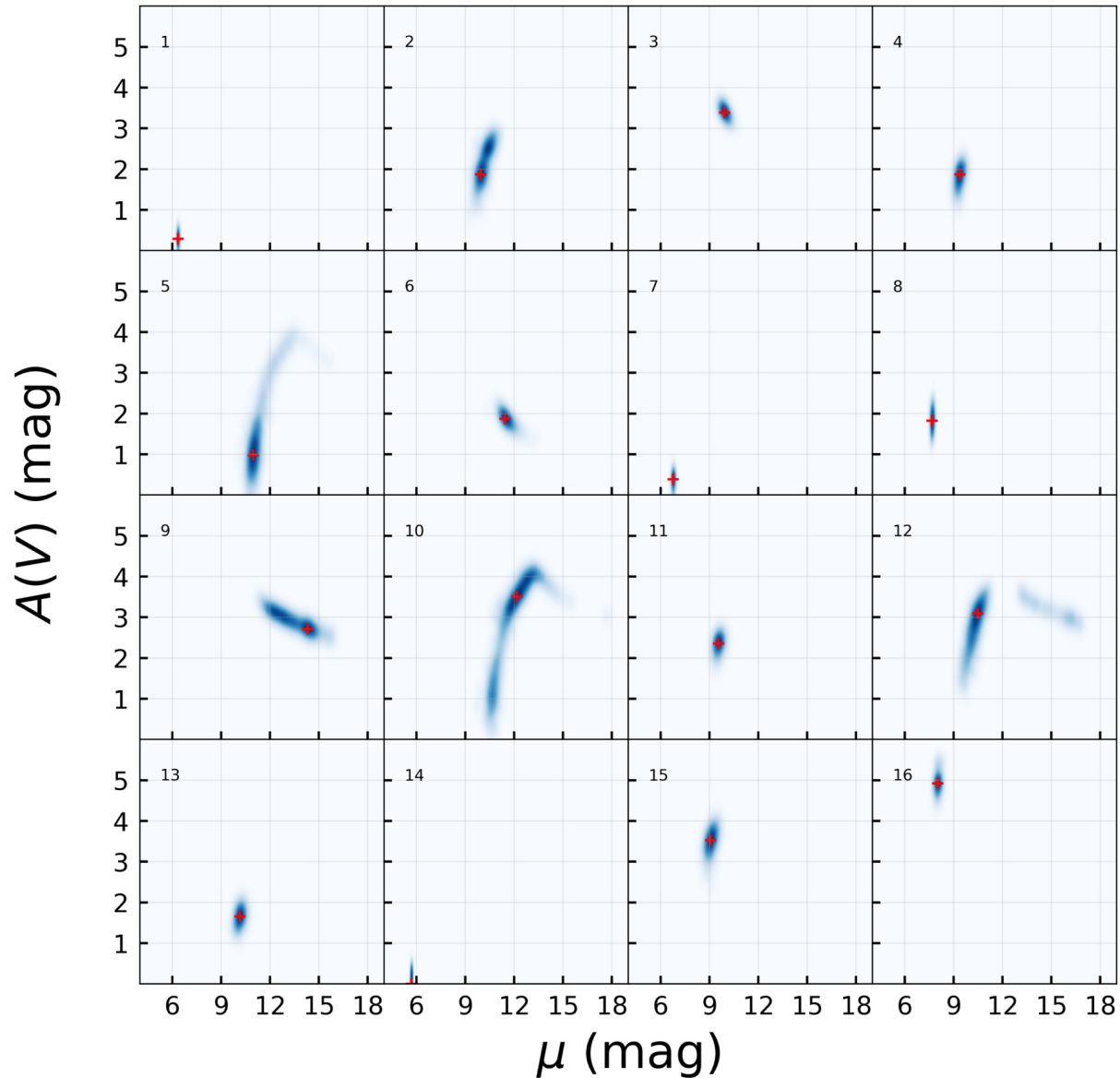
Figure 1. from A Large Catalog of Accurate Distances to Local Molecular Clouds: The Gaia DR2 Edition null 2019 APJ 879 125 doi:10.3847/1538-4357/ab2388 https://dx.doi.org/10.3847/1538-4357/ab2388 © 2019. The American Astronomical Society. All rights reserved.
