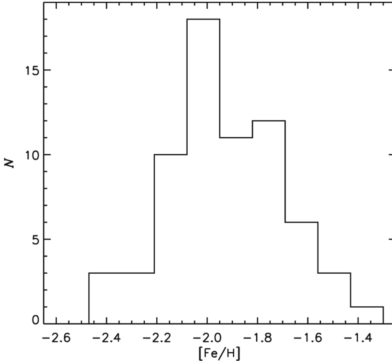
Figure 9. from Member Stars of the GD-1 Tidal Stream from the SDSS, LAMOST, and Gaia Surveys null 2019 APJ 877 13 doi:10.3847/1538-4357/ab158a https://dx.doi.org/10.3847/1538-4357/ab158a © 2019. The American Astronomical Society. All rights reserved.
