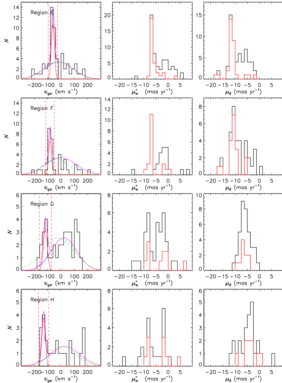
Figure 6. from Member Stars of the GD-1 Tidal Stream from the SDSS, LAMOST, and Gaia Surveys null 2019 APJ 877 13 doi:10.3847/1538-4357/ab158a https://dx.doi.org/10.3847/1538-4357/ab158a
