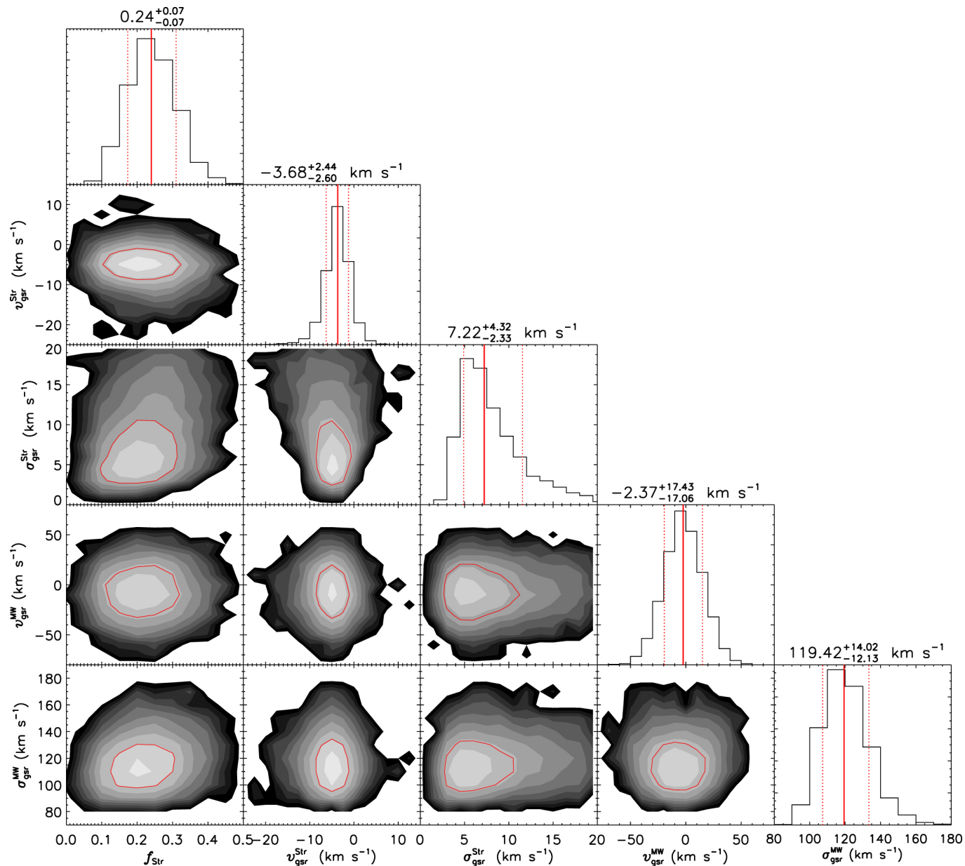
Figure 4. from Member Stars of the GD-1 Tidal Stream from the SDSS, LAMOST, and Gaia Surveys null 2019 APJ 877 13 doi:10.3847/1538-4357/ab158a https://dx.doi.org/10.3847/1538-4357/ab158a © 2019. The American Astronomical Society. All rights reserved.
