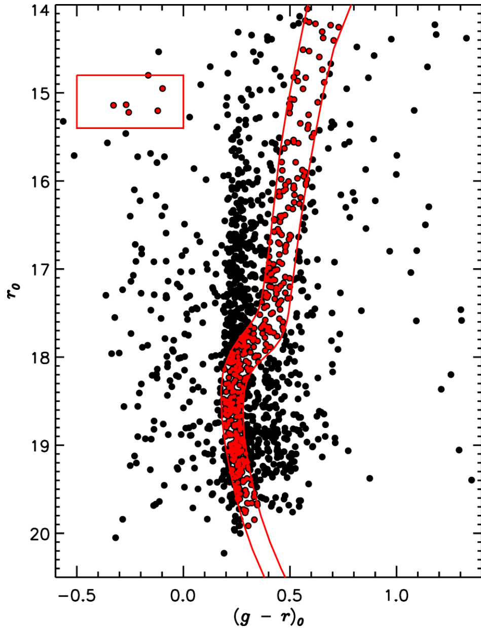
Figure 2. from Member Stars of the GD-1 Tidal Stream from the SDSS, LAMOST, and Gaia Surveys null 2019 APJ 877 13 doi:10.3847/1538-4357/ab158a https://dx.doi.org/10.3847/1538-4357/ab158a © 2019. The American Astronomical Society. All rights reserved.
