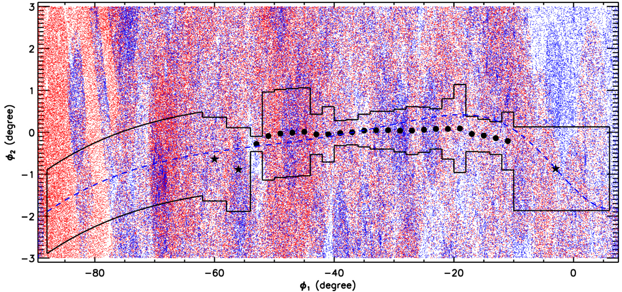
Figure 1. from Member Stars of the GD-1 Tidal Stream from the SDSS, LAMOST, and Gaia Surveys null 2019 APJ 877 13 doi:10.3847/1538-4357/ab158a https://dx.doi.org/10.3847/1538-4357/ab158a © 2019. The American Astronomical Society. All rights reserved.
