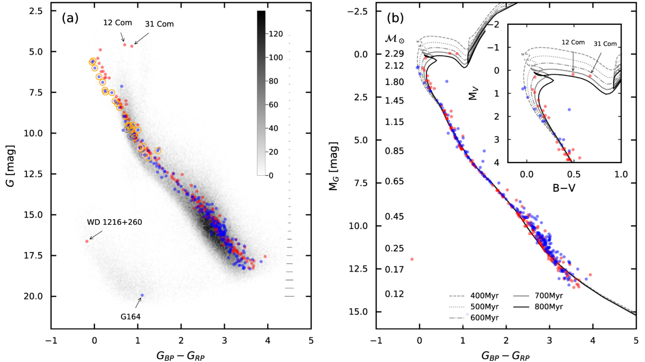
Figure 5. from Discovery of Tidal Tails in Disrupting Open Clusters: Coma Berenices and a Neighbor Stellar Group null 2019 APJ 877 12 doi:10.3847/1538-4357/ab13b0 https://dx.doi.org/10.3847/1538-4357/ab13b0 © 2019. The American Astronomical Society. All rights reserved.
