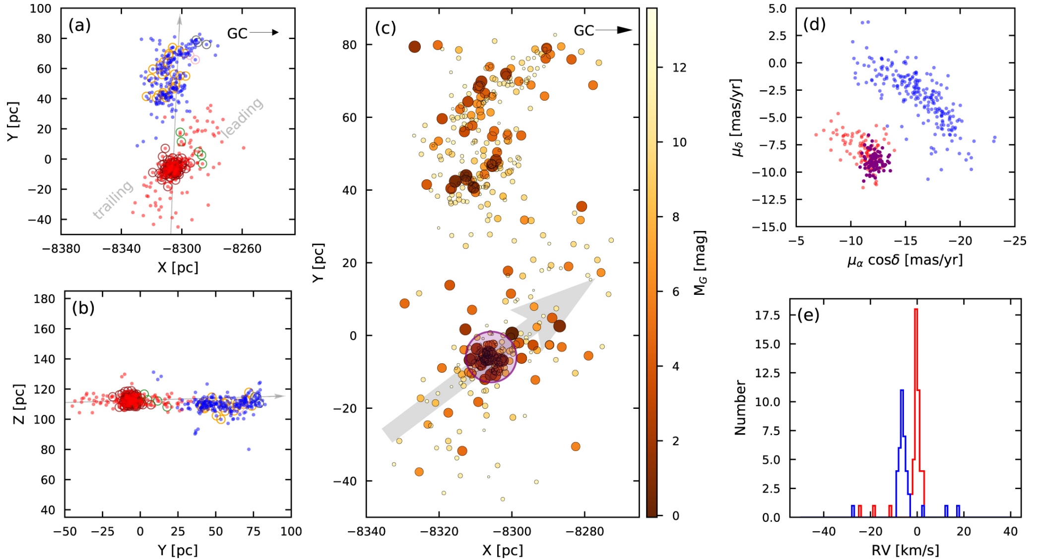
Figure 4. from Discovery of Tidal Tails in Disrupting Open Clusters: Coma Berenices and a Neighbor Stellar Group null 2019 APJ 877 12 doi:10.3847/1538-4357/ab13b0 https://dx.doi.org/10.3847/1538-4357/ab13b0 © 2019. The American Astronomical Society. All rights reserved.
