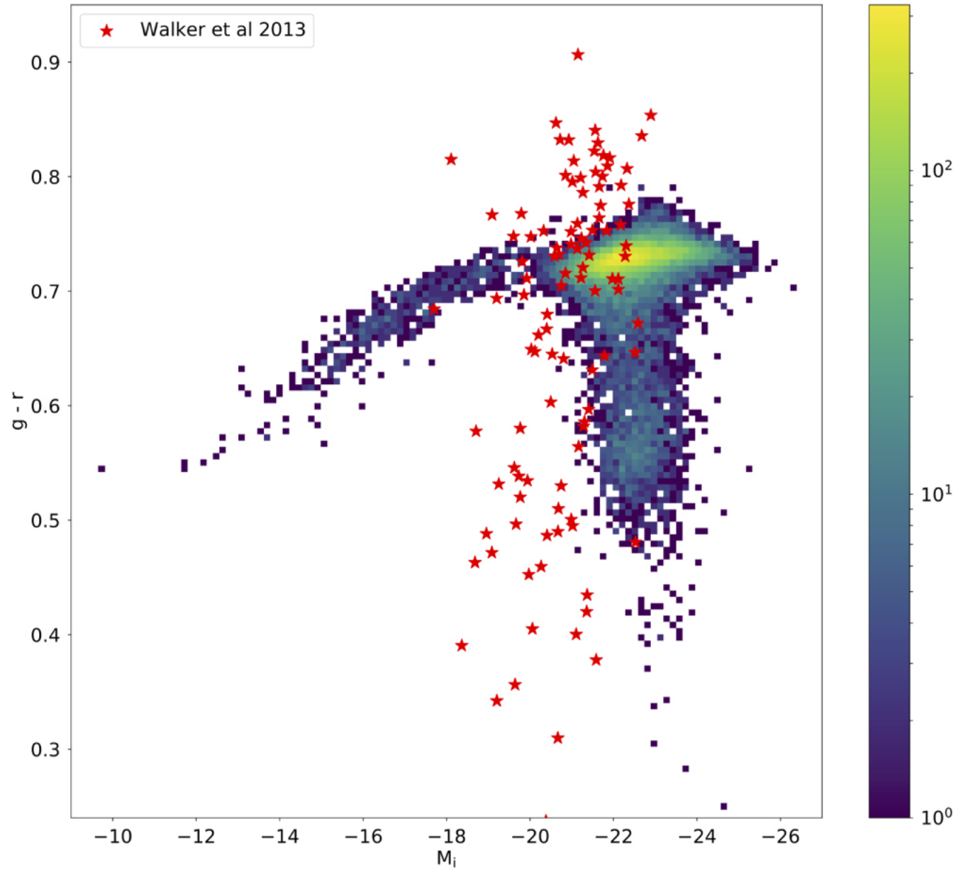
Figure 7. from The Occurrence of Compact Groups of Galaxies through Cosmic Time null 2019 APJ 873 124 doi:10.3847/1538-4357/ab053e https://dx.doi.org/10.3847/1538-4357/ab053e © 2019. The American Astronomical Society. All rights reserved.
