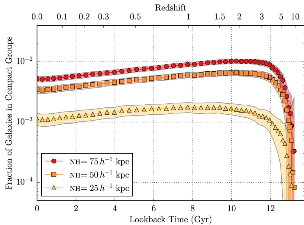
Figure 6. from The Occurrence of Compact Groups of Galaxies through Cosmic Time null 2019 APJ 873 124 doi:10.3847/1538-4357/ab053e https://dx.doi.org/10.3847/1538-4357/ab053e © 2019. The American Astronomical Society. All rights reserved.
