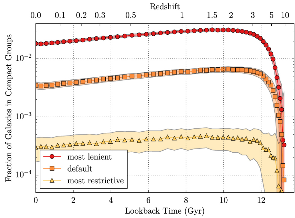
Figure 5. from The Occurrence of Compact Groups of Galaxies through Cosmic Time null 2019 APJ 873 124 doi:10.3847/1538-4357/ab053e https://dx.doi.org/10.3847/1538-4357/ab053e © 2019. The American Astronomical Society. All rights reserved.
