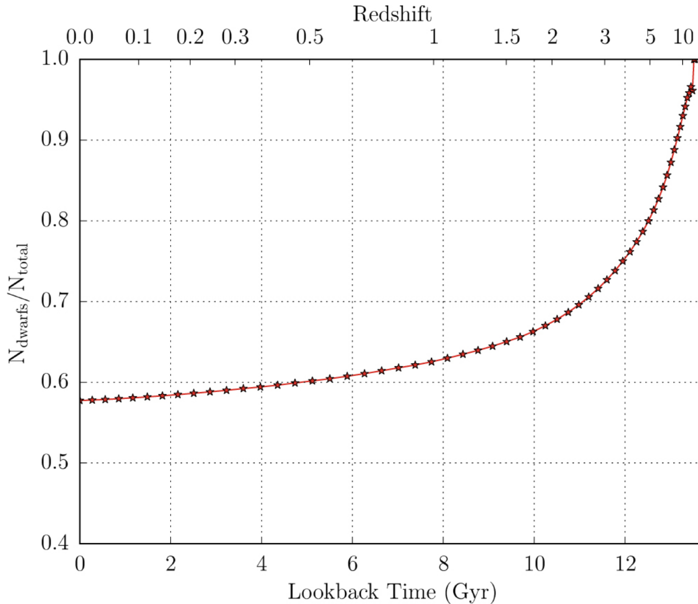
Figure 2. from The Occurrence of Compact Groups of Galaxies through Cosmic Time null 2019 APJ 873 124 doi:10.3847/1538-4357/ab053e https://dx.doi.org/10.3847/1538-4357/ab053e © 2019. The American Astronomical Society. All rights reserved.
