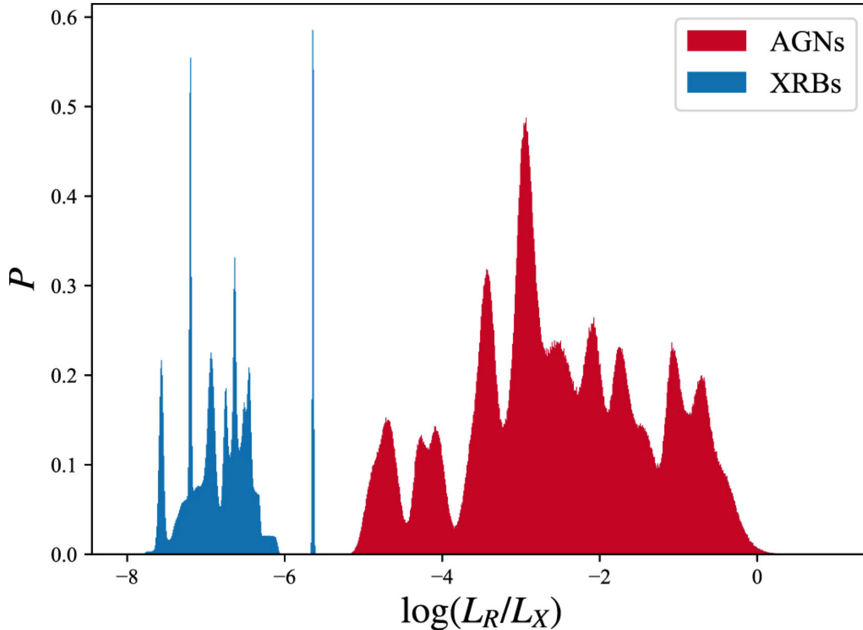
Figure 3. from The Fundamental Plane of Black Hole Accretion and Its Use as a Black Hole-Mass Estimator null 2019 APJ 871 80 doi:10.3847/1538-4357/aaf6b9 https://dx.doi.org/10.3847/1538-4357/aaf6b9 © 2019. The American Astronomical Society. All rights reserved.
