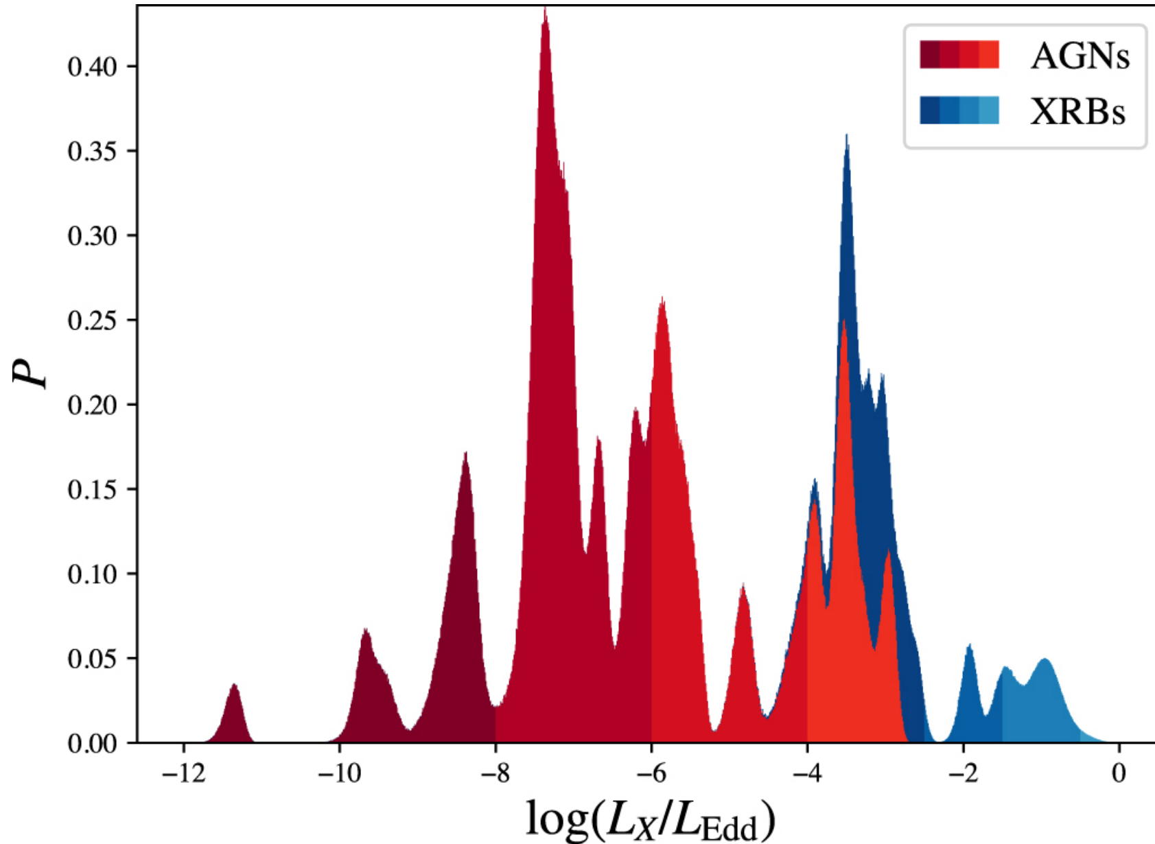
Figure 2. from The Fundamental Plane of Black Hole Accretion and Its Use as a Black Hole-Mass Estimator null 2019 APJ 871 80 doi:10.3847/1538-4357/aaf6b9 https://dx.doi.org/10.3847/1538-4357/aaf6b9 © 2019. The American Astronomical Society. All rights reserved.
