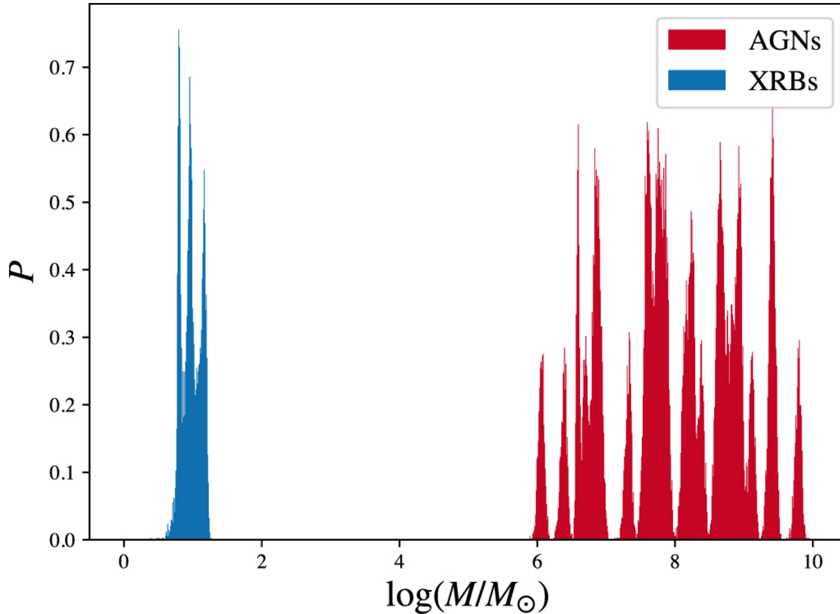
Figure 1. from The Fundamental Plane of Black Hole Accretion and Its Use as a Black Hole-Mass Estimator null 2019 APJ 871 80 doi:10.3847/1538-4357/aaf6b9 https://dx.doi.org/10.3847/1538-4357/aaf6b9 © 2019. The American Astronomical Society. All rights reserved.
