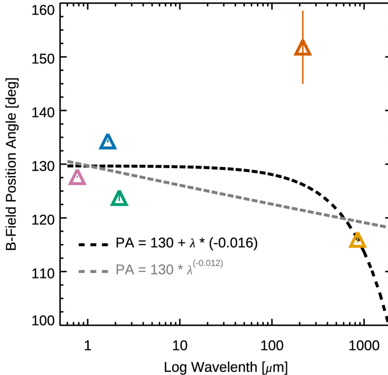
Figure 6. from Magnetic Field Uniformity Across the GF 9-2 YSO, L1082C Dense Core, and GF 9 Filamentary Dark Cloud null 2018 APJ 867 79 doi:10.3847/1538-4357/aae2af https://dx.doi.org/10.3847/1538-4357/aae2af © 2018. The American Astronomical Society. All rights reserved.
