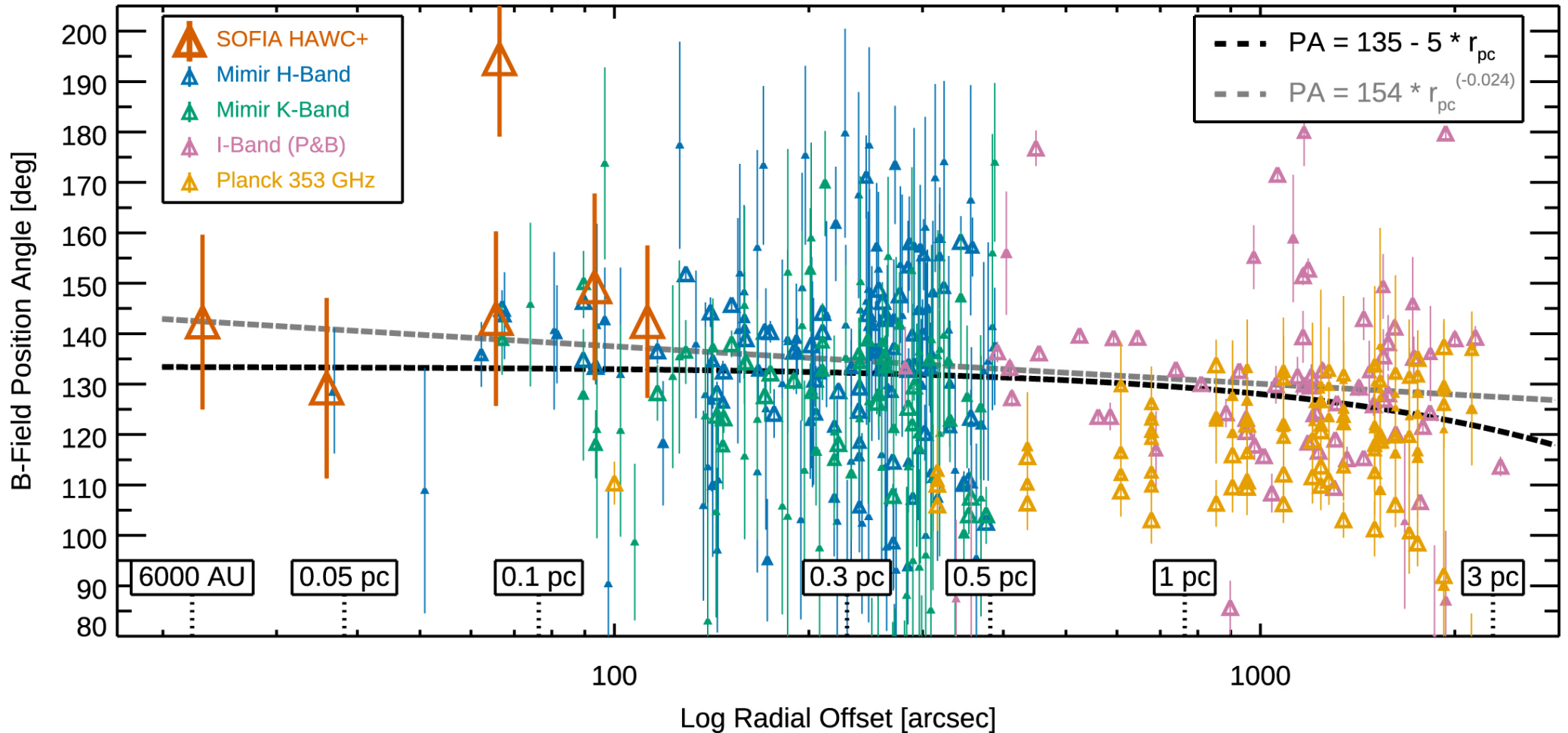
Figure 5. from Magnetic Field Uniformity Across the GF 9-2 YSO, L1082C Dense Core, and GF 9 Filamentary Dark Cloud null 2018 APJ 867 79 doi:10.3847/1538-4357/aae2af https://dx.doi.org/10.3847/1538-4357/aae2af © 2018. The American Astronomical Society. All rights reserved.
