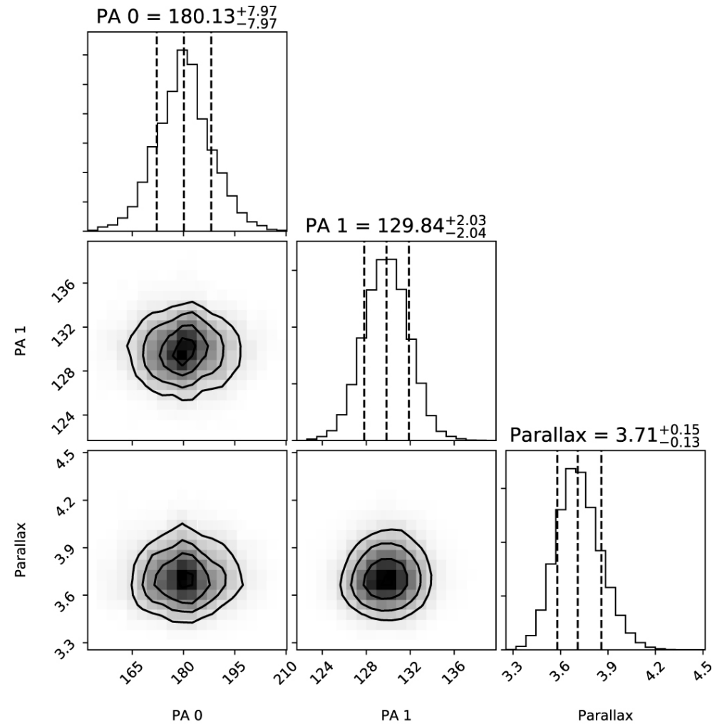
Figure 3. from Magnetic Field Uniformity Across the GF 9-2 YSO, L1082C Dense Core, and GF 9 Filamentary Dark Cloud null 2018 APJ 867 79 doi:10.3847/1538-4357/aae2af https://dx.doi.org/10.3847/1538-4357/aae2af © 2018. The American Astronomical Society. All rights reserved.
