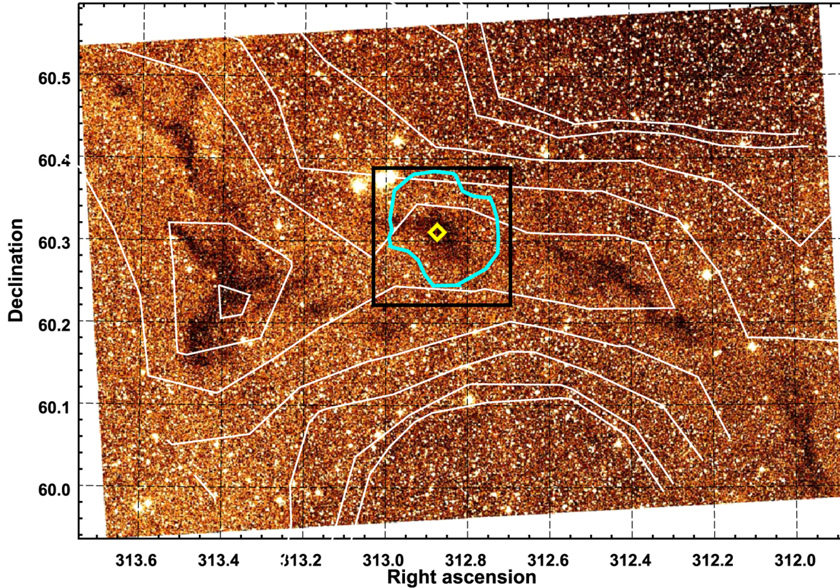
Figure 1. from Magnetic Field Uniformity Across the GF 9-2 YSO, L1082C Dense Core, and GF 9 Filamentary Dark Cloud null 2018 APJ 867 79 doi:10.3847/1538-4357/aae2af https://dx.doi.org/10.3847/1538-4357/aae2af © 2018. The American Astronomical Society. All rights reserved.
