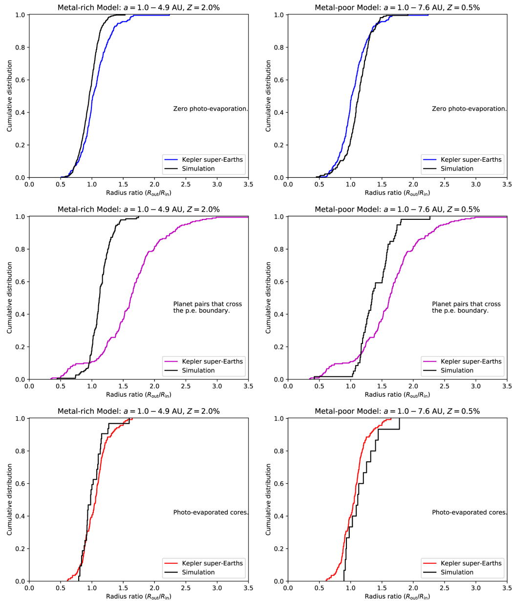
Figure 9. from Identifying Inflated Super-Earths and Photo-evaporated Cores null 2018 APJ 866 104 doi:10.3847/1538-4357/aadf8a https://dx.doi.org/10.3847/1538-4357/aadf8a © 2018. The American Astronomical Society. All rights reserved.
