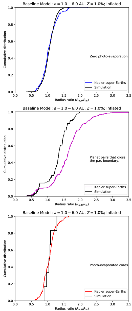
Figure 7. from Identifying Inflated Super-Earths and Photo-evaporated Cores null 2018 APJ 866 104 doi:10.3847/1538-4357/aadf8a https://dx.doi.org/10.3847/1538-4357/aadf8a © 2018. The American Astronomical Society. All rights reserved.
