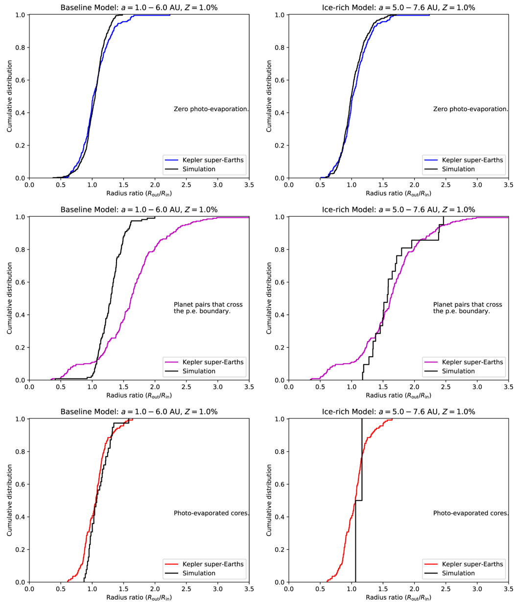
Figure 6. from Identifying Inflated Super-Earths and Photo-evaporated Cores null 2018 APJ 866 104 doi:10.3847/1538-4357/aadf8a https://dx.doi.org/10.3847/1538-4357/aadf8a © 2018. The American Astronomical Society. All rights reserved.
