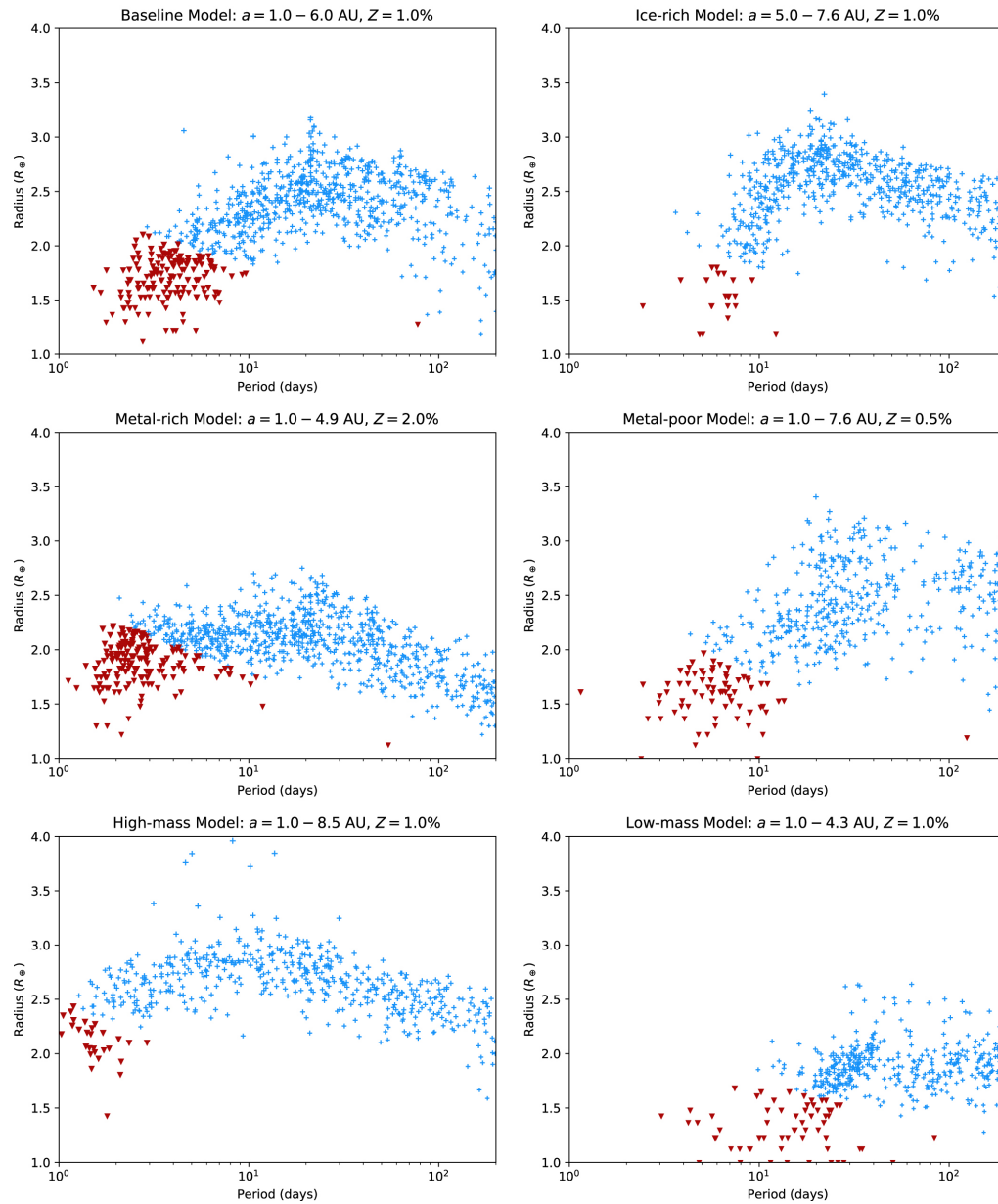
Figure 5. from Identifying Inflated Super-Earths and Photo-evaporated Cores null 2018 APJ 866 104 doi:10.3847/1538-4357/aadf8a https://dx.doi.org/10.3847/1538-4357/aadf8a © 2018. The American Astronomical Society. All rights reserved.
