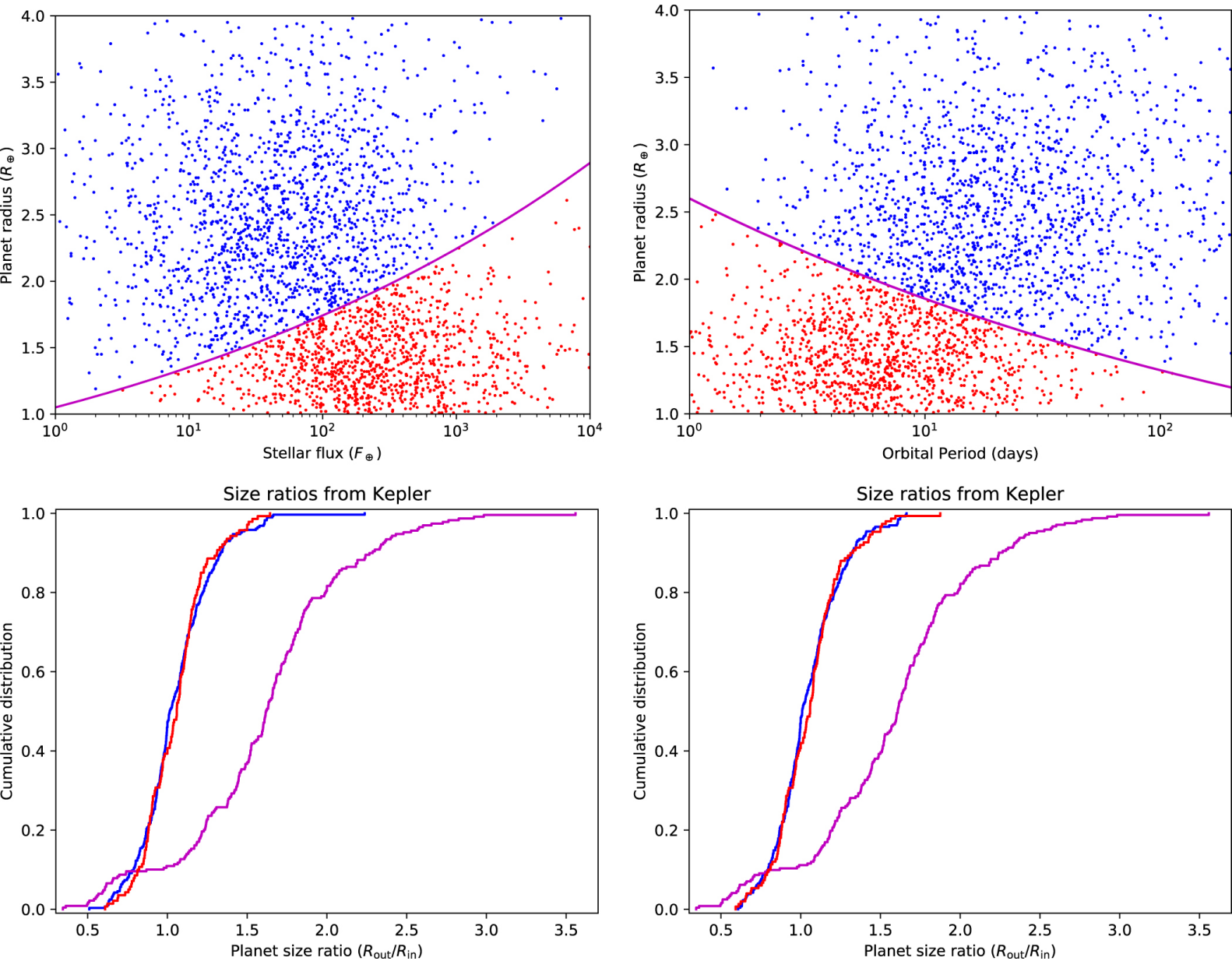
Figure 1. from Identifying Inflated Super-Earths and Photo-evaporated Cores null 2018 APJ 866 104 doi:10.3847/1538-4357/aadf8a https://dx.doi.org/10.3847/1538-4357/aadf8a © 2018. The American Astronomical Society. All rights reserved.
