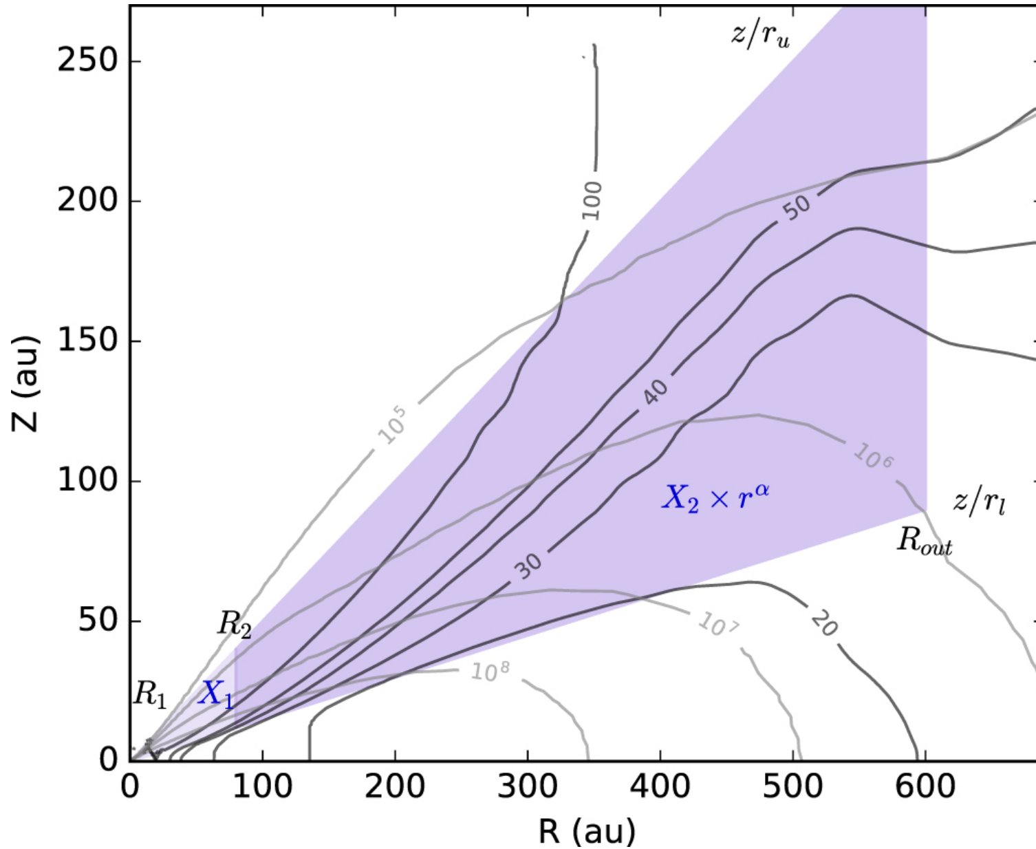
Figure 4. from H 2 CO Ortho-to-para Ratio in the Protoplanetary Disk HD 163296 null 2018 APJ 864 170 doi:10.3847/1538-4357/aad778 http://dx.doi.org/10.3847/1538-4357/aad778 © 2018. The American Astronomical Society. All rights reserved.
