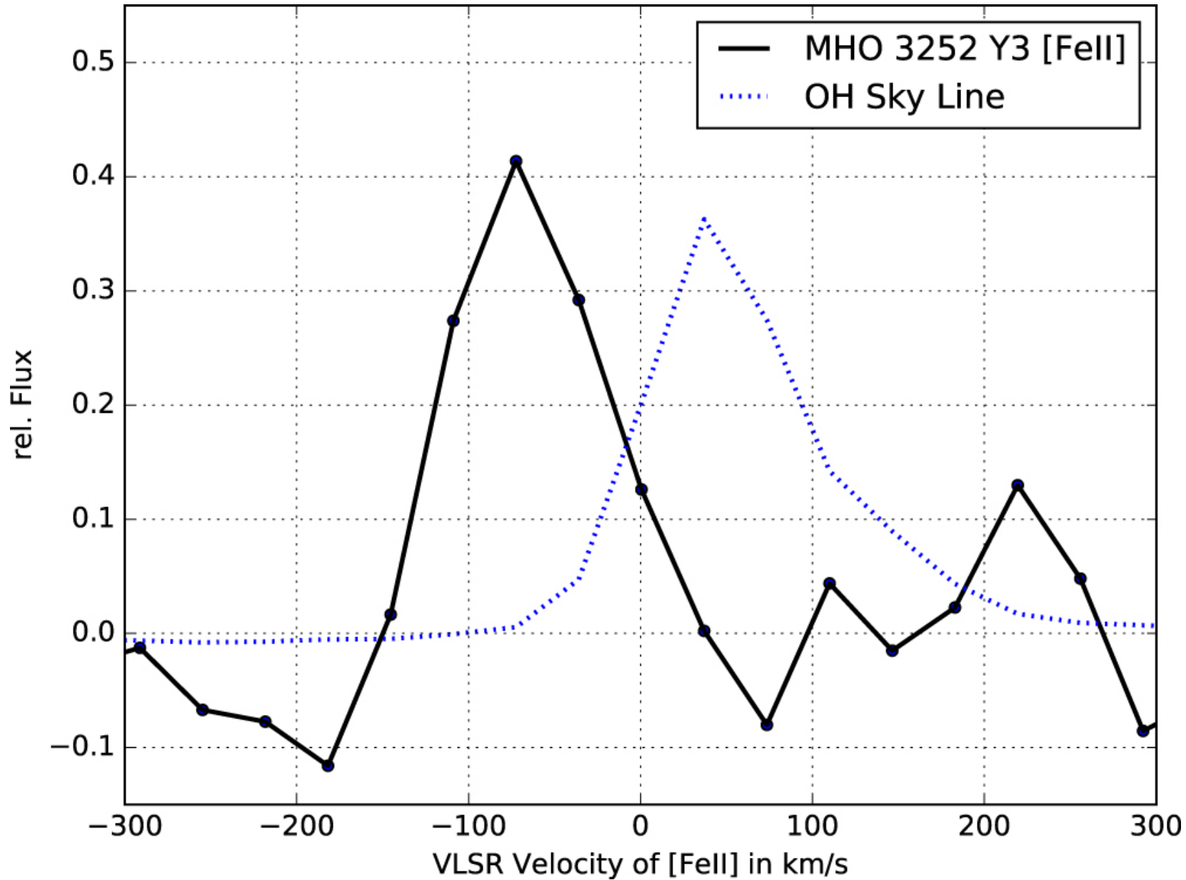
Figure 9. from Variability and Jet Activity in the YSO MHO 3252 Y3 in Serpens South null 2018 APJ 864 172 doi:10.3847/1538-4357/aad636 https://dx.doi.org/10.3847/1538-4357/aad636 © 2018. The American Astronomical Society. All rights reserved.
