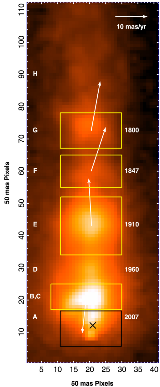
Figure 5. from Variability and Jet Activity in the YSO MHO 3252 Y3 in Serpens South null 2018 APJ 864 172 doi:10.3847/1538-4357/aad636 https://dx.doi.org/10.3847/1538-4357/aad636 © 2018. The American Astronomical Society. All rights reserved.
