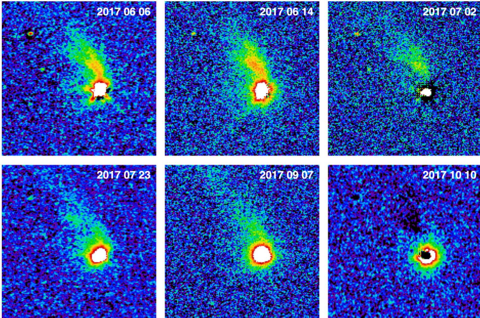
Figure 4. from Variability and Jet Activity in the YSO MHO 3252 Y3 in Serpens South null 2018 APJ 864 172 doi:10.3847/1538-4357/aad636 https://dx.doi.org/10.3847/1538-4357/aad636 © 2018. The American Astronomical Society. All rights reserved.
