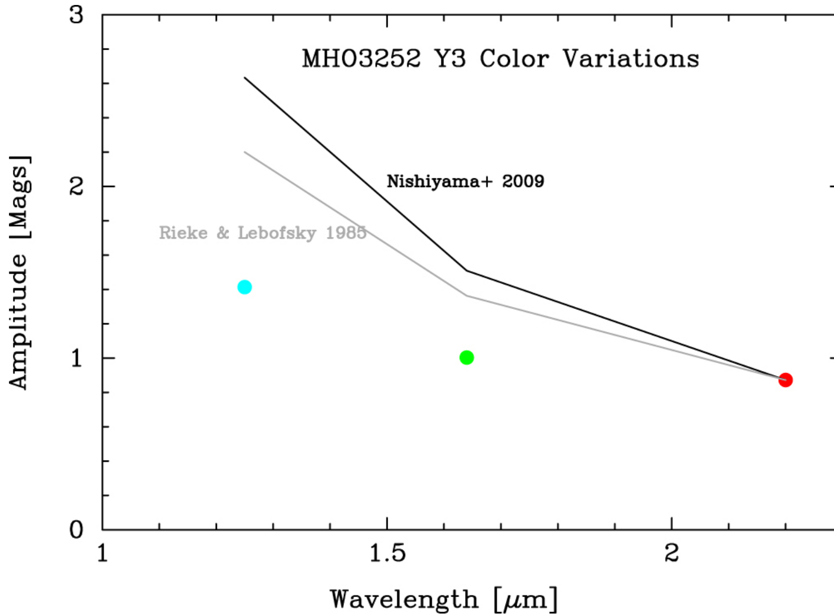
Figure 10. from Variability and Jet Activity in the YSO MHO 3252 Y3 in Serpens South null 2018 APJ 864 172 doi:10.3847/1538-4357/aad636 https://dx.doi.org/10.3847/1538-4357/aad636 © 2018. The American Astronomical Society. All rights reserved.
