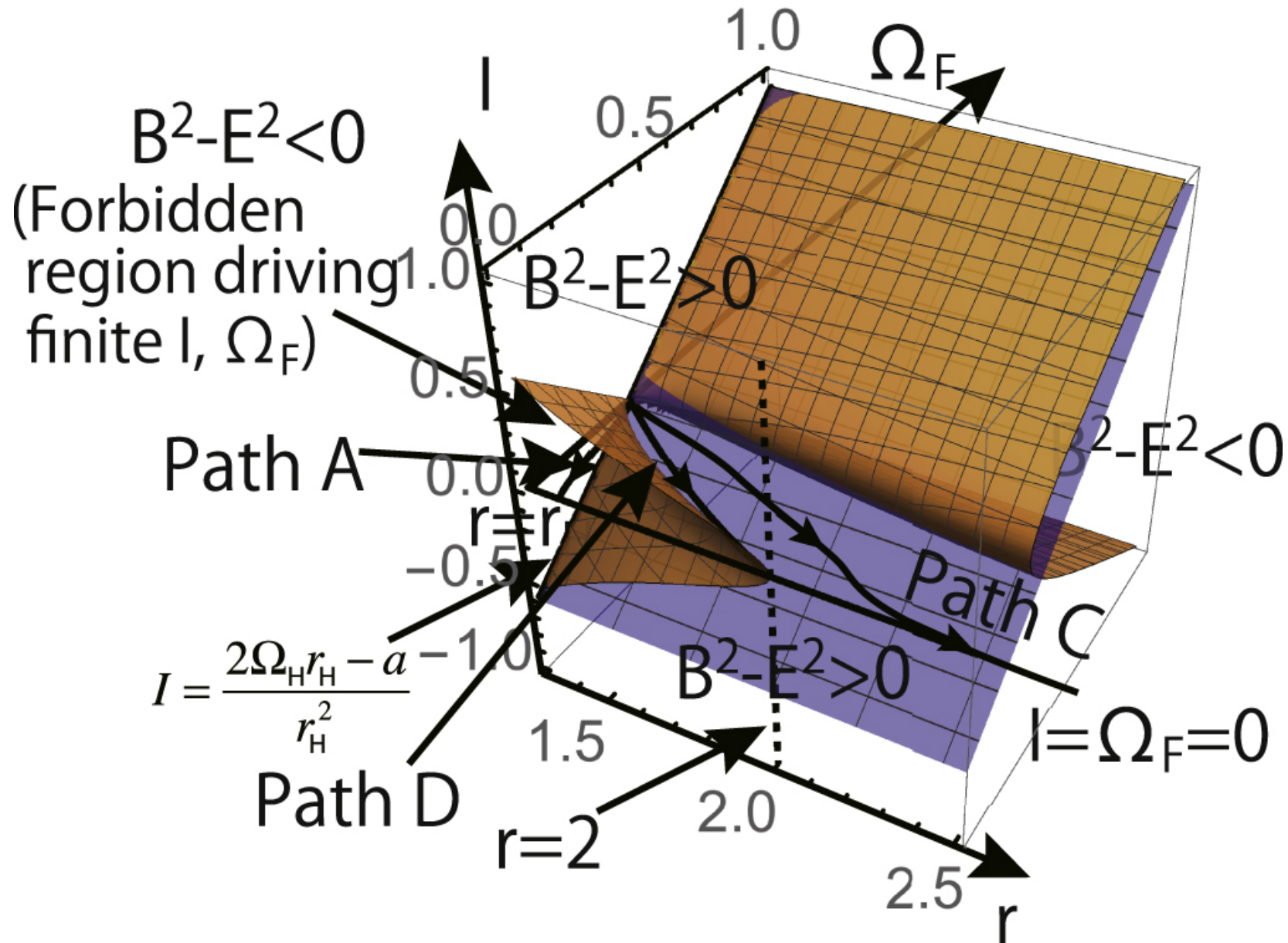
Figure 6. from Dynamic Process of Spontaneous Energy Radiation from Spinning Black Holes through Force-free Magnetic Field null 2018 APJ 864 173 doi:10.3847/1538-4357/aad4fe https://dx.doi.org/10.3847/1538-4357/aad4fe © 2018. The American Astronomical Society. All rights reserved.
