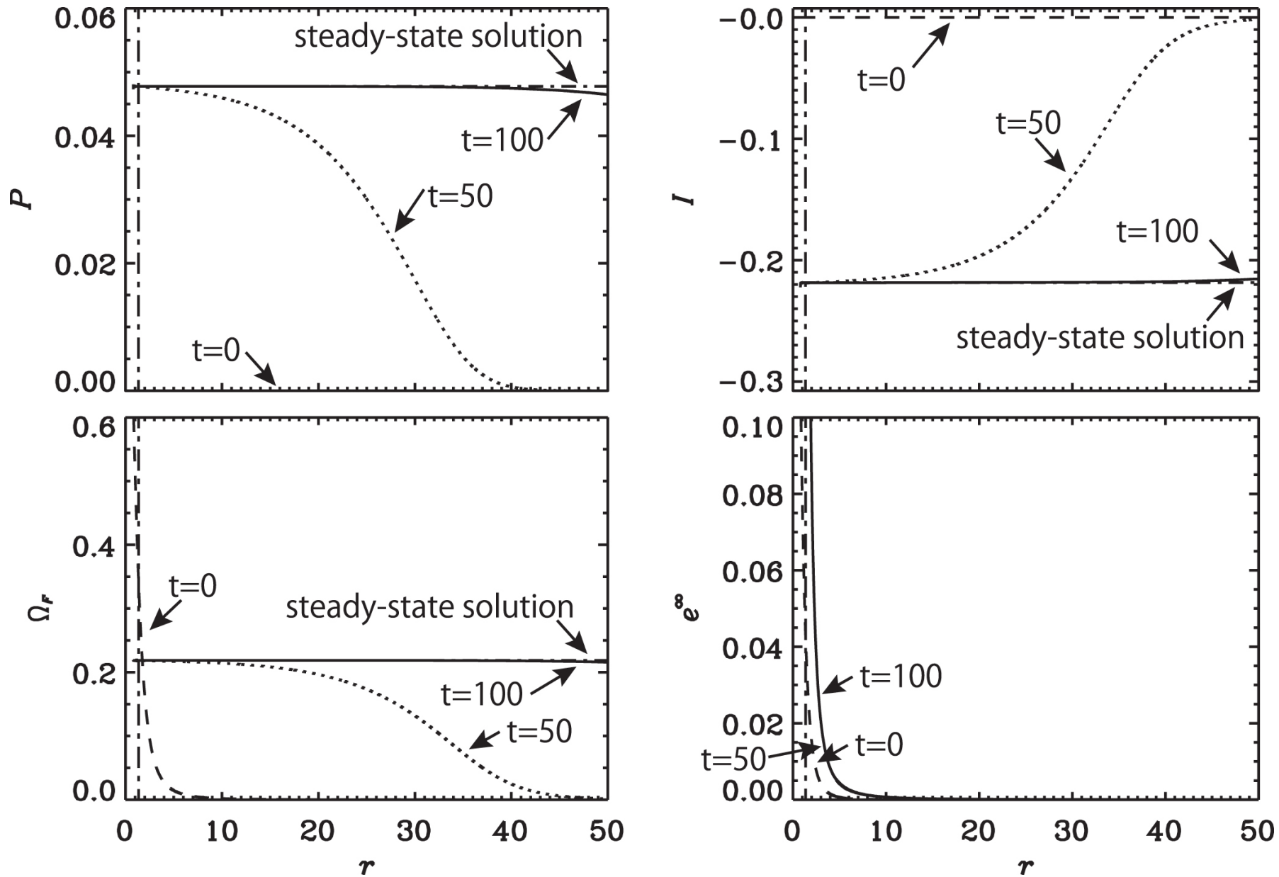
Figure 2. from Dynamic Process of Spontaneous Energy Radiation from Spinning Black Holes through Force-free Magnetic Field null 2018 APJ 864 173 doi:10.3847/1538-4357/aad4fe https://dx.doi.org/10.3847/1538-4357/aad4fe © 2018. The American Astronomical Society. All rights reserved.
