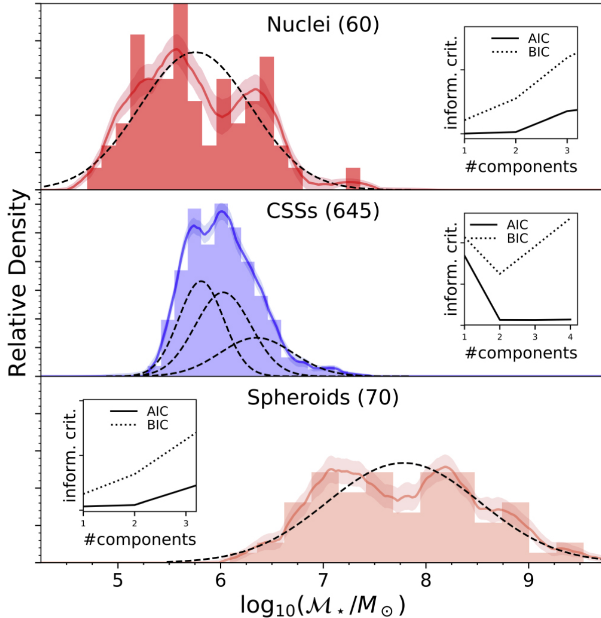
Figure 7. from The Next Generation Fornax Survey (NGFS). IV. Mass and Age Bimodality of Nuclear Clusters in the Fornax Core Region null 2018 APJ 860 4 doi:10.3847/1538-4357/aac1b8 https://dx.doi.org/10.3847/1538-4357/aac1b8 © 2018. The American Astronomical Society. All rights reserved.
