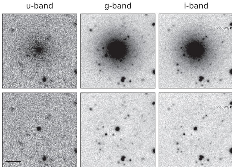
Figure 4. from The Next Generation Fornax Survey (NGFS). IV. Mass and Age Bimodality of Nuclear Clusters in the Fornax Core Region null 2018 APJ 860 4 doi:10.3847/1538-4357/aac1b8 https://dx.doi.org/10.3847/1538-4357/aac1b8 © 2018. The American Astronomical Society. All rights reserved.
