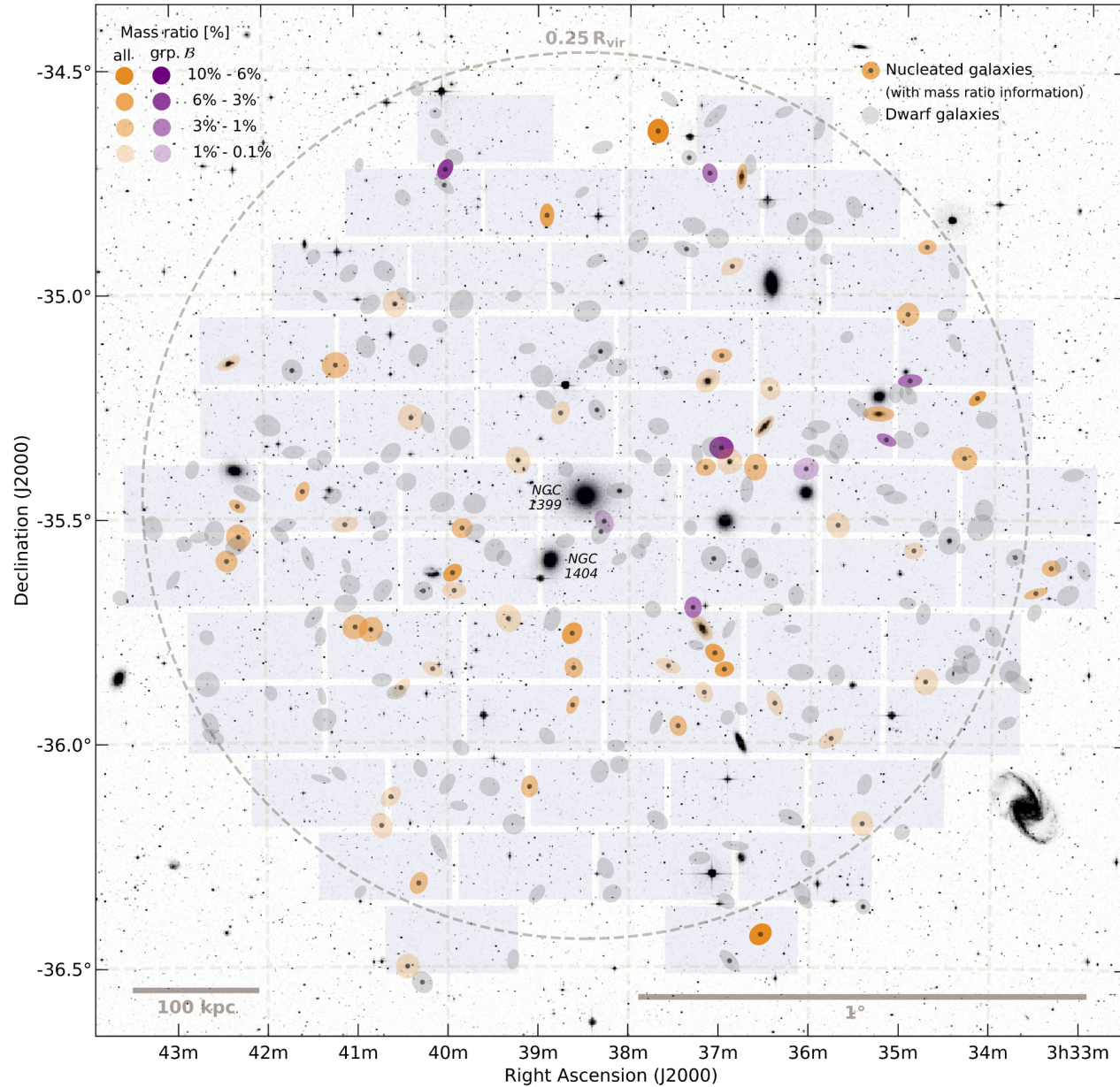
Figure 12. from The Next Generation Fornax Survey (NGFS). IV. Mass and Age Bimodality of Nuclear Clusters in the Fornax Core Region null 2018 APJ 860 4 doi:10.3847/1538-4357/aac1b8 https://dx.doi.org/10.3847/1538-4357/aac1b8 © 2018. The American Astronomical Society. All rights reserved.
